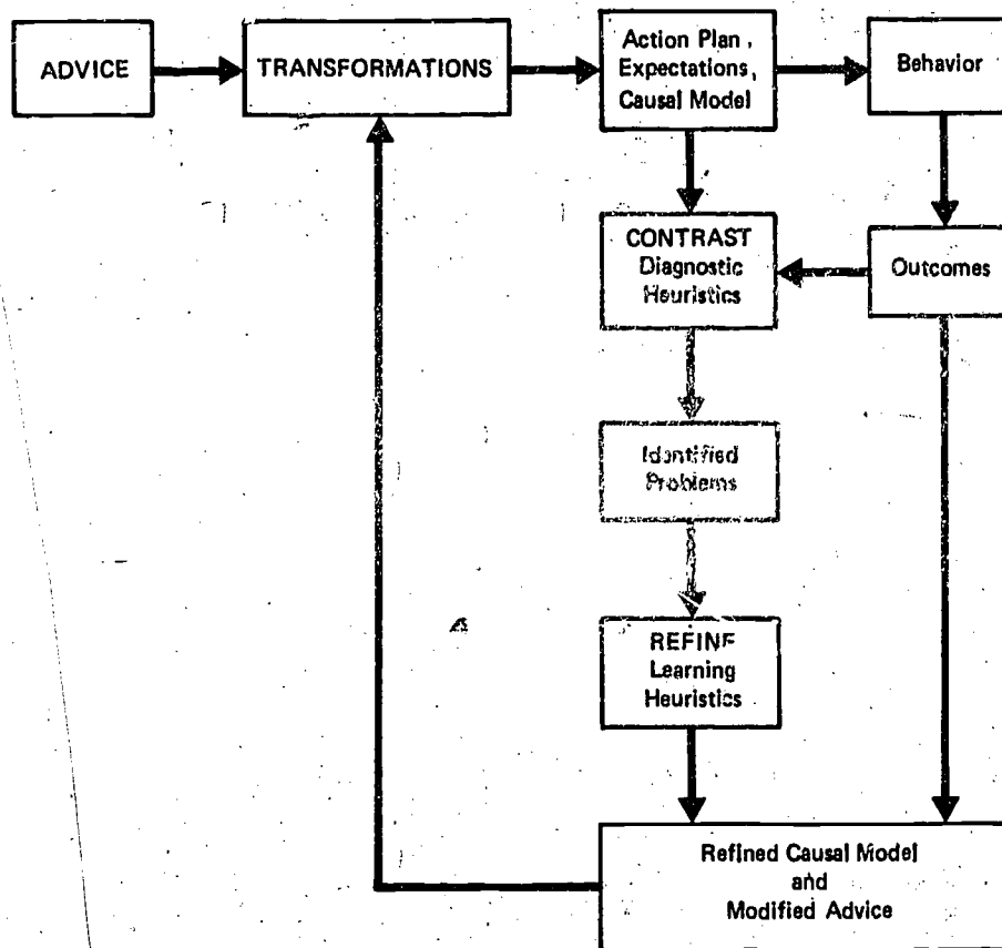
Fig. 4—Knowledge-refinement strategy
